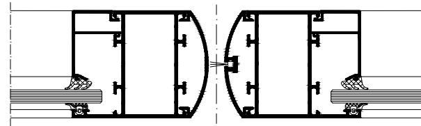
Pendelstulpprofil Swing door meeting stile profile
