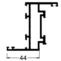
Tür-Z-Blendrahmenprofil Door Z-shaped outer frame profile
