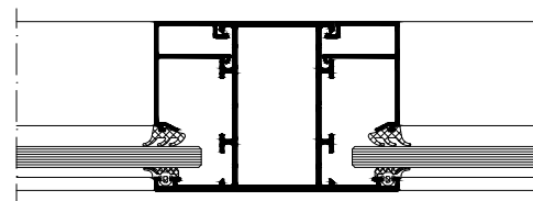
Riegel / Pfosten Transom/mullion
