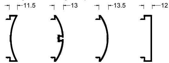
Pendelstulpprofil Swing door meeting stile profile
