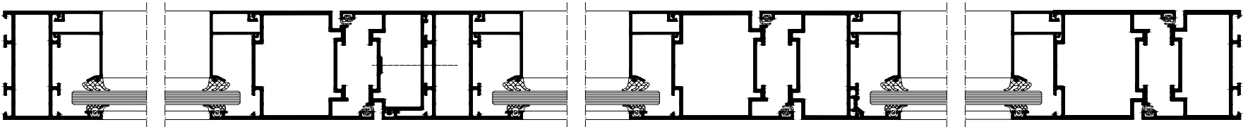
Pendeltür Swing door
