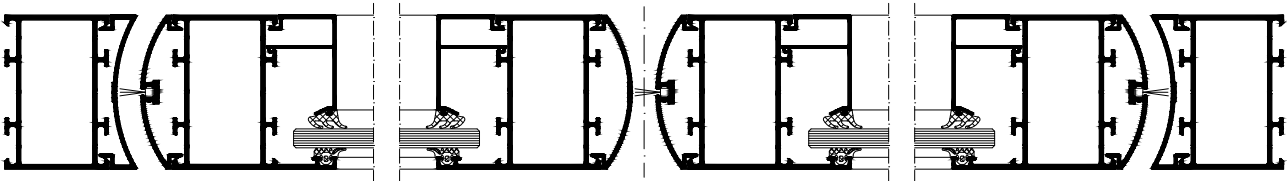
3 Pendeltür Swing door
