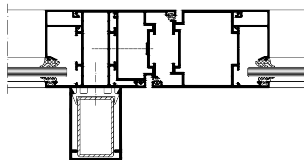
Statikpfosten Structural mullion
