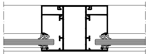
Riegel / Pfosten Transom/mullion
